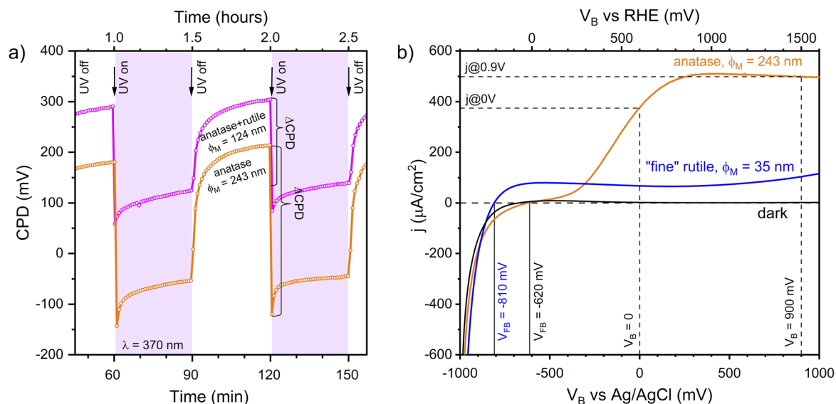
Fig. 8 Contact potential difference CPD vs. time for rutile/anatase and anatase thin films with changes under 370 nm illumination ( \Delta\text{CPD} ) marked (a); current density j as a function of applied bias voltage V_B in PEC (b).
