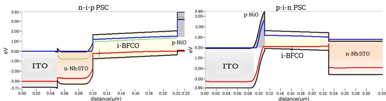
Fig. 15 Band alignment of simulated n-i-p and p-i-n PSCs, reproduced and adapted from Mahammedi et al. (2024) 96 ( https://doi.org/10.1016/j.jcleo.2024.171659 ) under a Creative Commons Attribution (CC BY 4.0) license.
