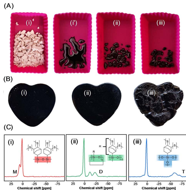
Fig. 12 (A) Melting behaviour of branch-poly( S-r -NBS20) with different degrees of siloxane branching. Granules of branch-poly( S-r -MENBS20) before (i) and after 2 h (i') at 80 °C. Granules of (ii) branch-poly( S-r -DCNBS20) and (iii) branch-poly( S-r -TCNBS20) after 2 h at 80 °C. (B) Moulded objects made from 2 g of branch-poly( S-r -NBS20) at 80 °C overnight. While (i) branch-poly( S-r -MENBS20) and (ii) branch-poly( S-r -DCNBS20) adopted the shape of the mould, branch-poly( S-r -TCNBS20) was still rubbery at 80 °C and did not fully adopt the shape of the mould. (C) 29 Si CP/MAS NMR spectra of (i) branch-poly( S-r -MENBS20), (ii) branch-poly( S-r -DENBS20), and (iii) branch-poly( S-r -TENBS20), showing characteristic peaks for M, D, and T siloxane bonds, respectively. The peak at 1.4 ppm present in each of the spectra corresponds to the trimethyl-substituted silicon atom stemming from the TMNBS comonomer. Reproduced with permission from Angew. Chem. Int. Ed. 2022, 61, e202114896. Copyright 2025, John Wiley and Sons.
