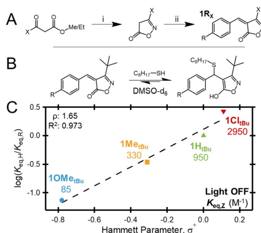
Fig. 2 (A) Synthesis of 1R_x acceptors: (i) ketoester, hydroxylamine, NaOAc, ethanol, 50 °C; (ii) isoxazolone, benzaldehyde, piperidine, isopropanol, 50 °C. (B) Equilibrium between 1R_{tBu} acceptors and OT. (C) Hammett plot of Z isomers of 1R_{tBu} acceptors versus the \sigma^+ Hammett parameter of R.
