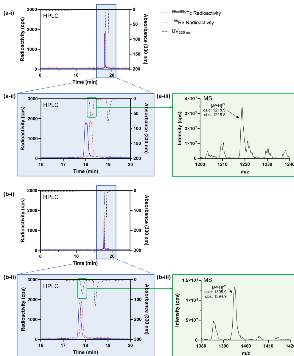
Fig. 5 (a-i) and (a-ii) UV chromatogram and radiochromatograms of reactions containing [\text{MO}_2(\text{DP}^{\text{An}}\text{-PSMAT})_2]^+ ( \text{M} = {}^{99\text{m}}\text{Tc} , {}^{99\text{m}}\text{Tc} or {}^{188}\text{Re} ); (a-iii) mass spectrum showing signal corresponding to [{}^{99\text{m}}\text{TcO}_2(\text{DP}^{\text{An}}\text{-PSMAT})_2]^+ . (b-i and b-ii) UV chromatogram and radiochromatograms of reactions containing [\text{MO}_2(\text{DP}^{\text{MEP}}\text{-PSMAT})_2]^+ ( \text{M} = {}^{99\text{m}}\text{Tc} , {}^{99\text{m}}\text{Tc} or {}^{188}\text{Re} ); (b-iii) mass spectrum showing signal corresponding to [{}^{99\text{m}}\text{TcO}_2(\text{DP}^{\text{MEP}}\text{-PSMAT})_2]^+ .
