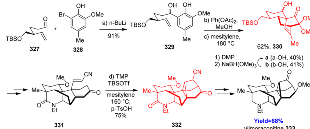
Scheme 42 Total synthesis of vilmoreaconitine (333). 94
