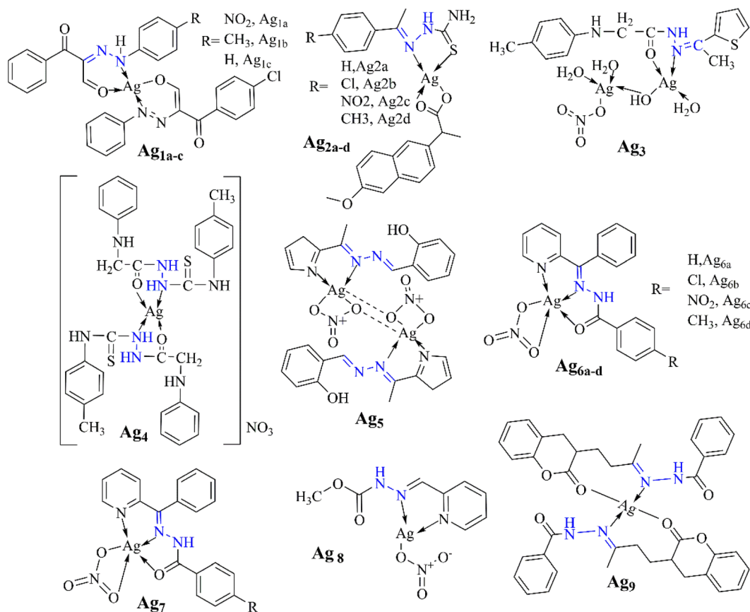
Fig. 14 Structure of some silver complexes ( Ag 1 –Ag 9 ). 86–94
