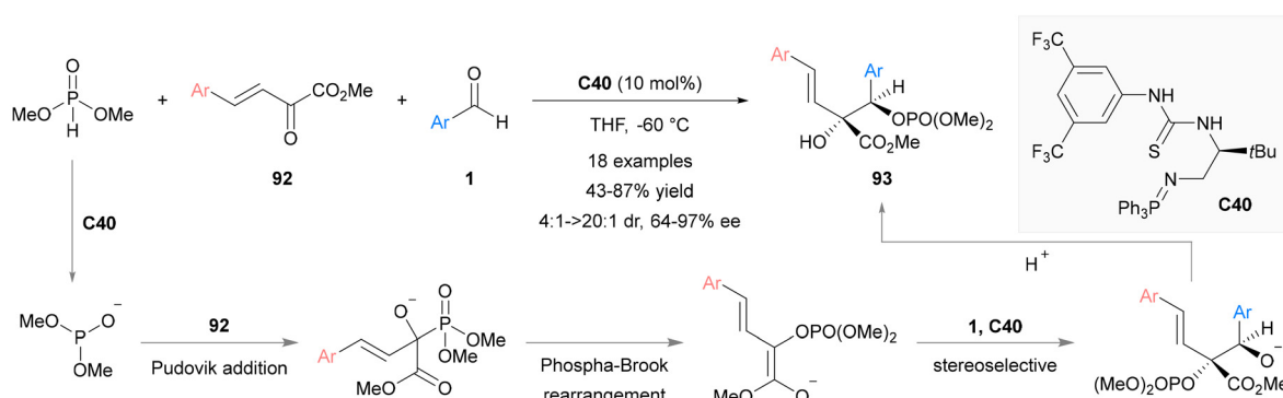
Fig. 21 Asymmetric reductive coupling reactions catalyzed by chiral thiourea.
