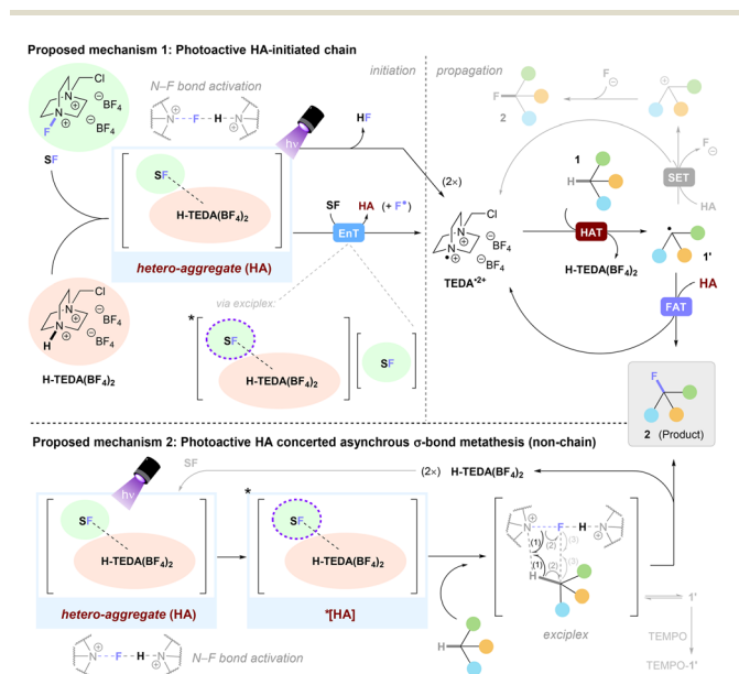
Scheme 5 Proposed reaction mechanisms.
