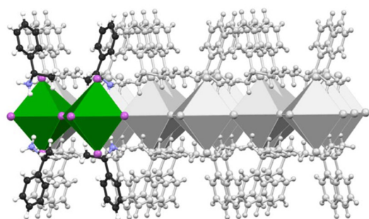
Scheme 1 Schematic representation of the investigated S\text{-MBA}_2\text{PbI}_4 structure under periodic boundary conditions. The unit cell used in the simulations comprises two metal–halide octahedra and four organic ligands, shown with coloured ball and stick models and polyhedra. A grey overlay illustrates the periodicity accounted for during the calculations.
