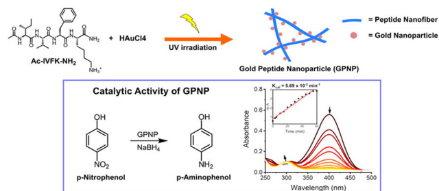
Fig. 11 Chemical structure of the tetramer peptide and the UV-assisted fabrication of GPNP composites (254 nm). The catalytic activity of GPNPs for the reduction of the small-molecule pollutant p -nitrophenol to the least toxic compound p -aminophenol, and the formation of p -aminophenol was detected simultaneously at around 400 nm, which indicates the catalytic activity of GPNP composites. Adapted with permission from ref. 170. Copyright 2022 American Chemical Society.
