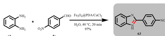
Scheme 31 Fe 3 O 4 @PDA/CuCl 2 for synthesis of benzimidazole (Badbedast et al. ).
