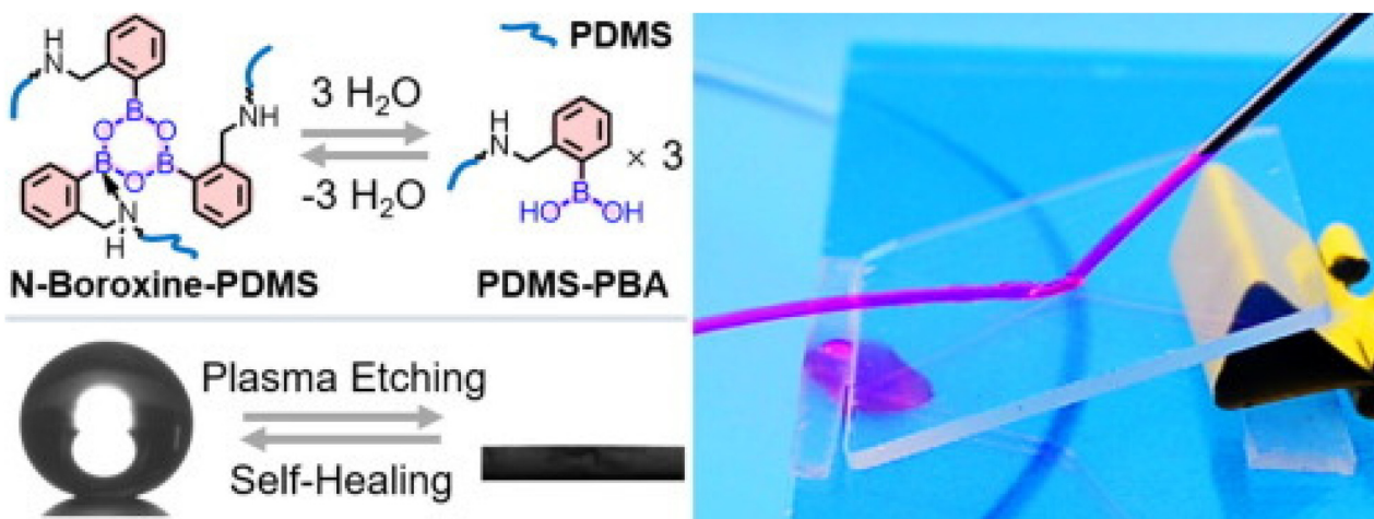
Fig. 14 Schematic of the formation of N -boroxine-PDMS from PDMS-PBA and images of an N -boroxine-PDMS transparent film. Reproduced with permission; 94 Copyright 2021, Elsevier.
