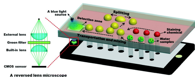
Fig. 47 Smartphone display-actuated optoelectrowetting droplet microfluidics for on-chip sample preparation and water quality detection. (A) Schematic overview of the digital microfluidic operations and (B) video frames showing these operations. (C) Smartphone-acquired fluorescent image of marine water sample showing target algae cells. The scale bar is 100 \mu\text{m} . Adapted from ref. 568 Copyright 2018 Royal Society of Chemistry.
