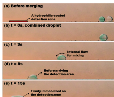
Fig. 47 Smartphone display-actuated optoelectrowetting droplet microfluidics for on-chip sample preparation and water quality detection. (A) Schematic overview of the digital microfluidic operations and (B) video frames showing these operations. (C) Smartphone-acquired fluorescent image of marine water sample showing target algae cells. The scale bar is 100 \mu\text{m} . Adapted from ref. 568 Copyright 2018 Royal Society of Chemistry.
