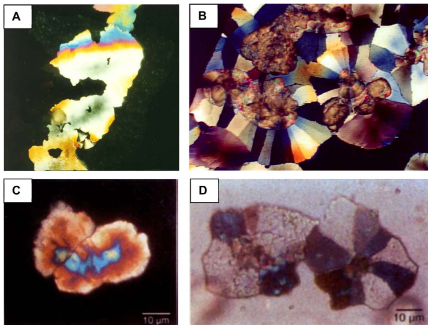
Fig. 4 Comparison between \text{CaCO}_3 films produced by the PILP process using polyaspartate (Na-salt) additive (A) and (B) versus \text{CaCO}_3 films produced using proteins extracted from nacre (C) and (D). (A) and (B) The PILP \text{CaCO}_3 films are typically about a half a micron in thickness, which is an ideal thickness for examining with polarized light microscopy. The color gradients arise from interference colors across variations in thickness, but upon rotation, the whole film patch exhibited a single-crystalline extinction direction. (C) and (D) Belcher's paper on "Control of crystal phase switching and orientation by soluble mollusc-shell proteins" 35 was primarily focused on how the proteins caused a shift from calcite to aragonite phase. However, it is notable that these extracted proteins, when used as additives with \text{CaCO}_3 precipitated in vitro , led to single crystalline patches of calcite film with non-equilibrium morphologies, very similar to the PILP model system (A) vs. (C). The polycrystalline patches of film contained a centralized 3D aggregate, which appeared to somehow modulate the orientation of the underlying single-crystalline "tablets" into a radiating pattern (B) vs. (D). (A) and (B) Reproduced from ref. 34, Copyright © 2008, American Chemical Society. (C) and (D) Reproduced from ref. 35, Copyright © 1996, Springer Nature Limited.
