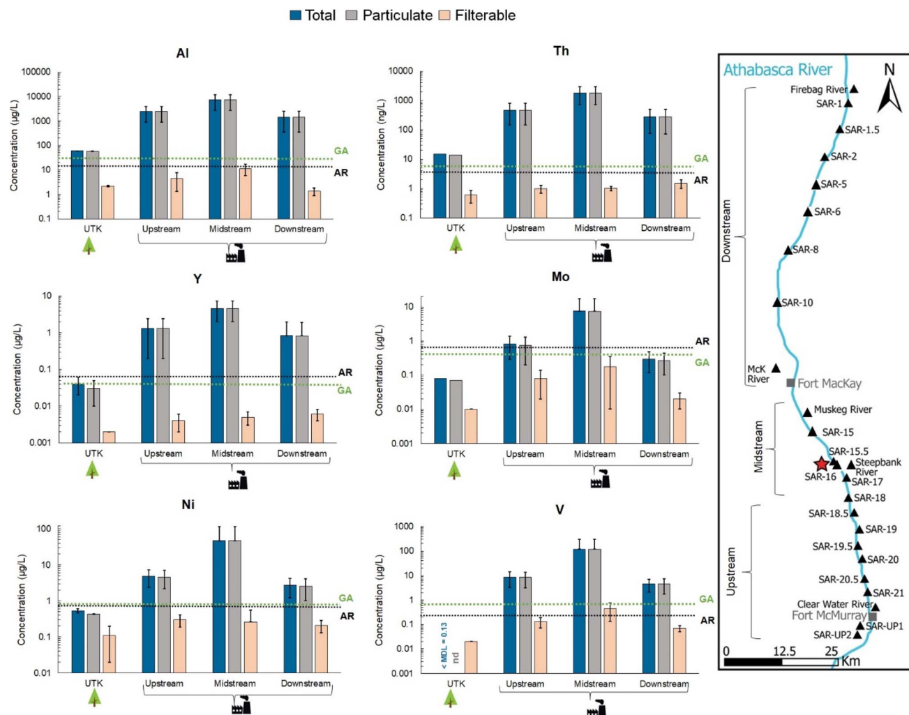
Fig. 2 Average concentrations of total, particulate and filterable ( <0.45 \mu\text{m} ) Al, Th, Y (conservative lithophile elements), Mo, Ni, and V (elements enriched in bitumen) in snow from upstream, midstream, and downstream locations (with respect to the industry), and at the reference site (UTK), winter 2016. The horizontal black line represents the dissolved TE concentrations in the AR main stem in autumn of 2014 (ref. 36) whereas the green line represents the global average (GA) dissolved ( <0.2 or 0.45 \mu\text{m} ) concentrations of TEs in river water. 64 Notes: the map on the right side shows the snow sampling locations in the ABS region along the Athabasca River (SAR) and its tributaries. The location of UTK is provided in Fig. S1 and Table S1 (SI). The red star represents the midpoint between bitumen upgraders. Error bars represent one standard deviation. LOD = limit of detection, MDL = method detection limit, nd = not determined. Th and Mo concentrations at UTK are based on one location instead of the average of two.
