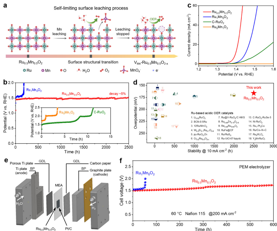
Fig. 1 Comparison of activity and stability of various catalysts. (a) Schematic illustration of the self-limiting surface leaching process. (b) Chronopotentiometric curves of Ru 0.5 Mn 0.5 O 2 , Ru 1 MnO 2 , Ru 0 MnO 2 , and C-RuO 2 at a current density of 10 mA cm -2 in 0.5 M H 2 SO 4 solution. (c) Polarization curves of Ru 0.5 Mn 0.5 O 2 , Ru 1 MnO 2 , Ru 0 MnO 2 , and C-RuO 2 . (d) Comparison of the overpotentials and stabilities for Ru 0.5 Mn 0.5 O 2 and recently reported Ru-based OER catalysts in acid media. (e) Schematic diagram of the PEM electrolyzer. A typical PEM electrolyzer consists of bipolar plates (BPs), gas diffusion layers (GDLs), and membrane electrode assembly (MEA). (f) Chronopotentiometry testing of PEM electrolyzers using Ru 0.5 Mn 0.5 O 2 or Ru 1 MnO 2 as the anodic catalyst and commercial Pt/C as the cathodic catalyst operated at 200 mA cm -2 at 60 °C.
