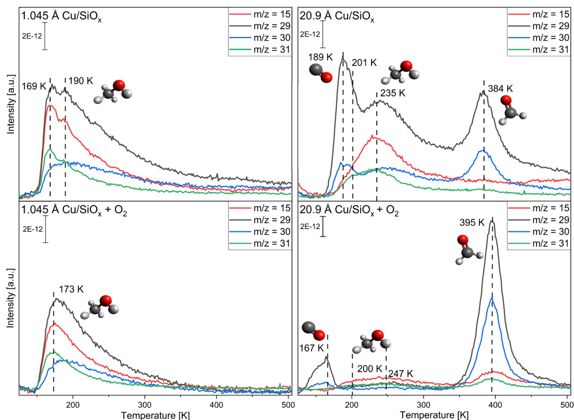
Fig. 2 Copper-coverage-dependent TPR spectra of a monolayer methanol (top spectra) adsorbed at T = 115 K and methanol with 56 L of oxygen pre-adsorbed (bottom spectra) on \text{SiO}_x . Shown are the relevant m/z signals for methanol ( m/z = 31 ), formaldehyde ( m/z = 29, 30 ) and methane ( m/z = 15 ), as well as some contributions from the carbon monoxide isotope desorption ( m/z = 29, 30 ). The desorption spectra are presented for 1.045 Å of copper (left) and 20.9 Å (right) of copper deposited. The heating rate of the sample is 2 \text{ K s}^{-1} .
