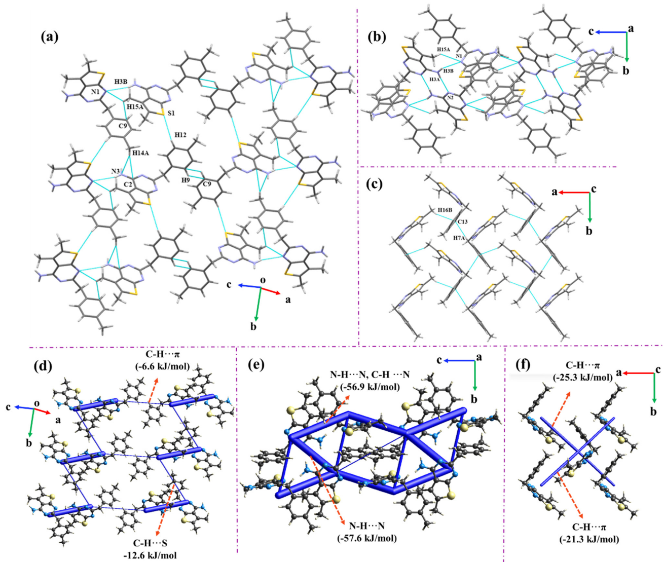
Fig. 7 (a) Crystal packing down the b -axis involving C-H \cdots S/ \pi interactions in compound 7; (b) herringbone pattern generated through dimeric N-H \cdots N and C-H \cdots N interactions in the bc -plane; (c) crystal packing through C-H \cdots \pi along the a -axis; (d)–(f) energy framework diagrams depicting the total energy component.
