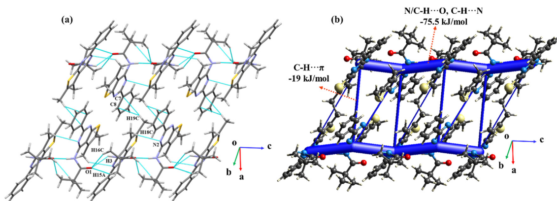
Fig. 8 (a) Infinite chains formed through N-H \cdots O, C-H \cdots O, and C-H \cdots N hydrogen bonds in compound 9. (b) Energy framework diagram depicting C-H \cdots O and C-H \cdots N interactions and their total energetic contributions.
