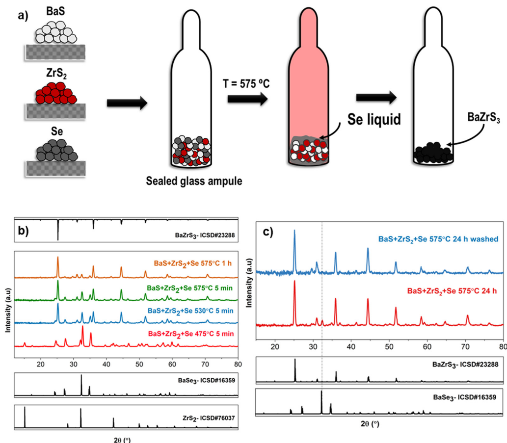
Fig. 8 (a) Reaction schematic depicting the synthesis of \text{BaMS}_3 utilizing a selenium liquid flux. (b) X-ray diffraction patterns illustrating the evolution of intermediate phases with temperature for binary sulfides when subjected to the selenium liquid flux. (c) Comparison plot of the X-ray diffraction pattern for the water-washed and unwashed \text{BaZrS}_3 powder.
