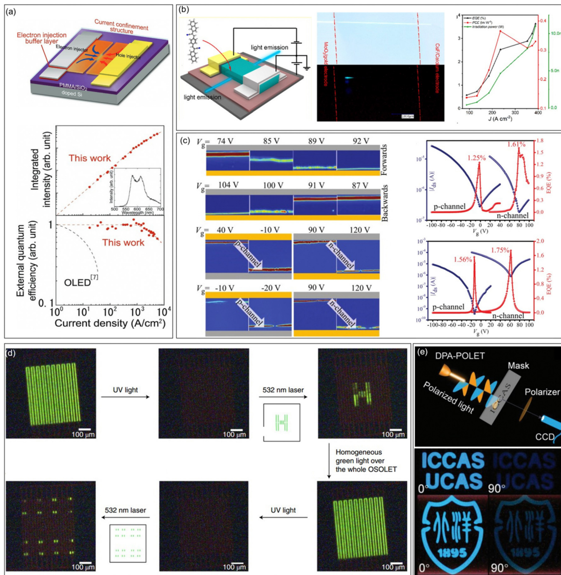
Fig. 8 Representative applications in OLETs. (a) Design principle for an improved organic single-crystal light emitting transistor with extremely high current density and current-density dependence of the integrated intensity of the luminescence spectra (top) and external quantum efficiency (bottom) in the ambipolar BP3T-OLETs. Reproduced with permission. 129 Copyright 2012, John Wiley and Sons. (b) Device structure of PBNA-based single crystal OLETs, photographs of the green crystal under natural light (upper) and electrical driving (lower) in OLETs, and the EQE, PCE, and irradiation power changes as a function of current density. Reproduced with permission. 108 Copyright 2021, American Chemical Society. (c) A series of color-coded images for 2,6-DPA and 2,6-DNA-based OLETs extracted from light emission captured by CCD operating under forward and backward, and EQE versus V_g for 2,6-DPA-OLET and 2,6-DNA-OLET within both p- and n-channel regions. Reproduced with permission. 130 Copyright 2019, John Wiley and Sons. (d) Emitting pattern created and erased within single OLETs. Reproduced with permission. 132 Copyright 2019, Springer Nature. (e) Schematic of the imaging system with DPA-OPLET as the light source and the images of imaging by DPA-OPLET with polarization angles of 0^\circ (left pictures) and 90^\circ (right pictures). Reproduced with permission. 133 Copyright 2023, John Wiley and Sons.
