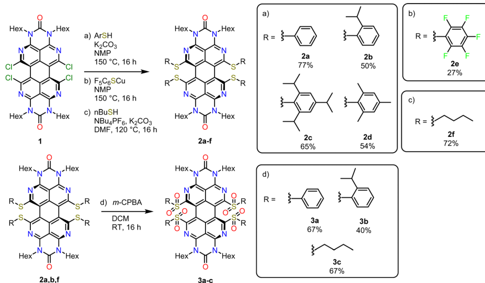
Scheme 1 Synthesis of thioether- and sulfone-functionalized OAPPDOs. Reaction conditions: (a) ArSH, \text{K}_2\text{CO}_3 , NMP, 150^\circ\text{C} , 16 h; (b) \text{F}_5\text{C}_6\text{SCu} , NMP, 150^\circ\text{C} , 16 h; (c) n\text{-BuSH} , \text{NBu}_4\text{PF}_6 , \text{K}_2\text{CO}_3 , DMF, 120^\circ\text{C} , 16 h; (d) m\text{-CPBA} , DCM, room temperature, 16 h.
