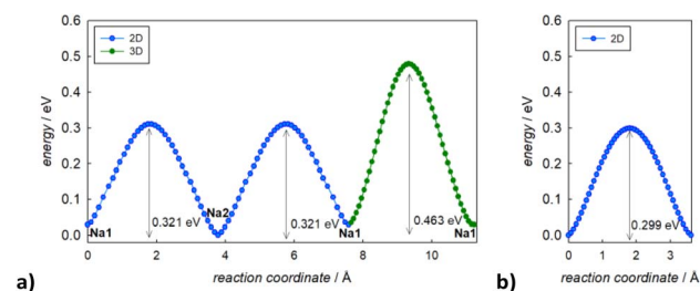
Fig. 3 Migration energy profiles as derived from BVSE analysis of the synchrotron diffraction data for tetragonal \text{Na}_3\text{SbS}_4 (a) and cubic \text{Na}_{2.9}\text{Sb}_{0.9}\text{W}_{0.1}\text{S}_4 (b).
