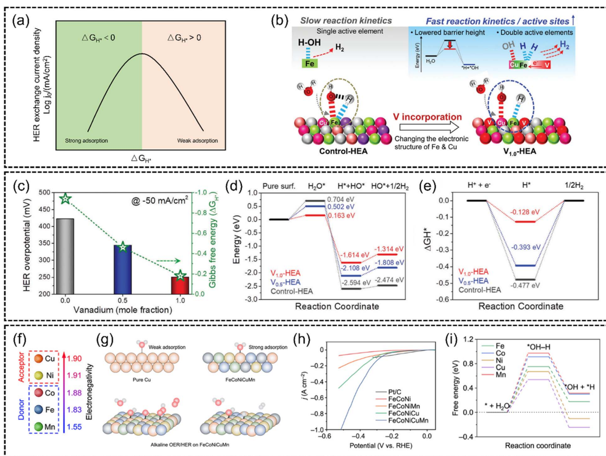
Fig. 11 (a) Schematic representation of a HER volcano plot exchange current \log j_0 versus adsorption free energy of hydrogen ( \Delta G_{\text{H}^*} ). (b) Schematic representation of the effect of vanadium incorporation on the barrier height and active sites at the surface of V_{1.0} -HEA. The V incorporation adjusts the electron structure of Fe and Cu elements, lowering the water dissociation energy and increasing active sites. (c) Activity (at -50 \text{ mA cm}^{-2} ) versus Gibbs free energy ( \Delta G_{\text{H}^*} ) relationship. (d) Reaction energy diagram of water dissociation. (e) Gibbs free energy ( \Delta G_{\text{H}^*} ) diagram of the surface of three HEAs. Reproduced with permission. 137 Copyright 2023, Wiley-VCH GmbH. (f) A comparison of the electronegativity of the elements Cu, Ni, Co, Fe and Mn. (g) Scheme of the different adsorption strengths of intermediates on metal sites in HEAs and Cu catalysts and reaction pathways of the alkaline HER and OER at the Cu sites in the HEA NPs. (h) HER polarization curves of the FeCoNi/CNF, FeCoNiMn/CNF, FeCoNiCu/CNF, and FeCoNiCuMn HEA/CNF catalysts in 1 \text{ M KOH} . (i) Gibbs free energy ( \Delta G_{\text{H}^*} ) profiles for the HER at the Fe, Co, Ni, Cu, and Mn sites. Reproduced with permission. 141 Copyright Royal Society of Chemistry 2023.
