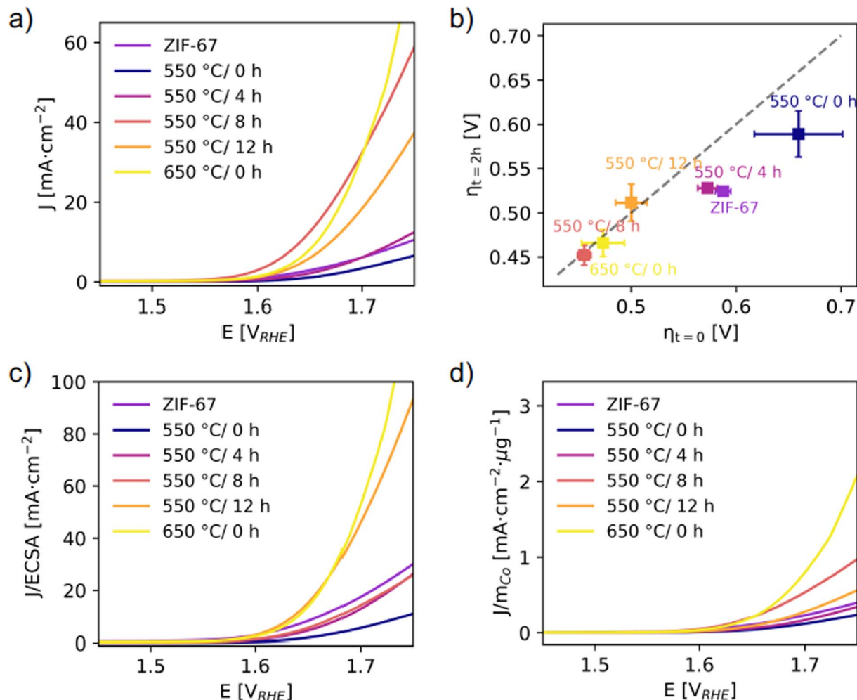
Fig. 7 (a) Linear sweep voltammety with a scan rate of 10 \text{ mV s}^{-1} . (b) Overpotentials were determined from chronopotentiometry at J = 10 \text{ mA cm}^{-2} per geometric area. The x-axis represents the overpotential at time t = 0 , as a measure of activity. The y-axis represents the overpotential at time t = 2 \text{ h} . The diagonal dashed line is the expected response for a stable catalyst, and deviations from this indicate an unstable catalyst. 51 (c) LSV responses normalized to the ECSA (from capacitance measurements, see Fig. S43†). (d) LSV responses normalized to the mass of cobalt calculated considering the final Co wt% after pyrolysis under the assumption that the mass loss during pyrolysis is entirely associated to the (volatile) organic linker (Fig. S48†).
