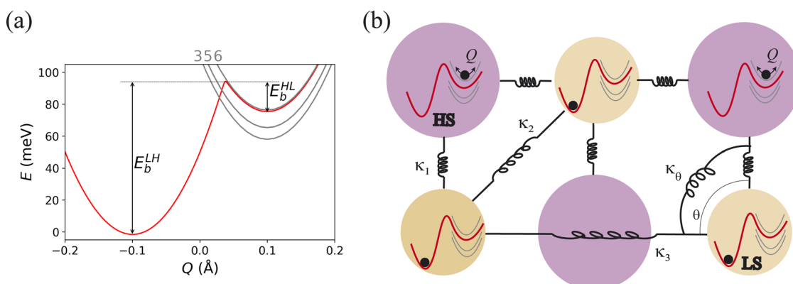
Fig. 2 Schematic of the model. (a) Each molecule is described by potential energy surfaces, V_s(Q) , derived from crystal field theory. Spin–orbit coupling is included perturbatively, allowing the intermediate spin term to be integrated out. This results in a double well (red), and fourteen pure HS levels (grey; degeneracies as labelled). The barriers E_b^{HL} and E_b^{LH} that regulate the single molecular kinetics are labelled. Only the breathing mode, Q , is considered explicitly, with the other molecular vibrations included only by their entropic contributions. (b) Molecules form a square lattice with elastic intermolecular interactions, \kappa_n , defined in eqn (S1–S3).†
