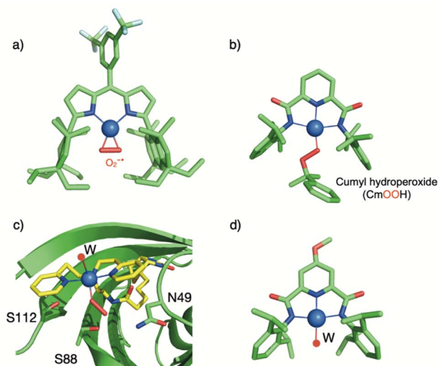
Fig. 6 Selected crystallographic structures of recently described mononuclear copper-oxygen adducts. a) \eta^2 -superoxo based on the ^{\text{EMind}}\mathbf{L} ligand. 83 Hydrogen atoms were omitted for clarity; b) The anion [(L)Cu(OOCm)] - based on the bis(arylcarboxamido)-pyridine ligand. 85 Hydrogen atoms and the Et 4 N + counter ion were omitted for clarity; c) \eta^1 -Hydroperoxido complex in an artificial enzyme based on a streptavidin scaffold: [(biot-et-dpea)Cu II (OOH)(OH 2 )] + c Sav; 86 d) High-valent [(L)CuOH] species based on the bis(arylcarboxamido)-pyridine ligand (W as deprotonated water ligand). 87
