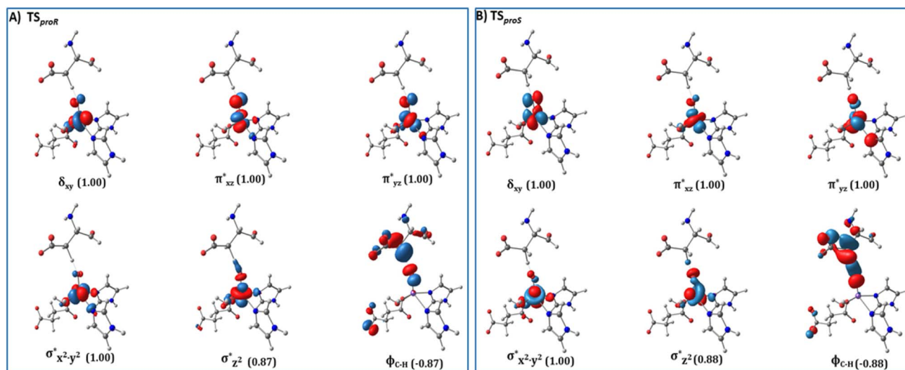
Fig. 6 Spin Natural Orbitals (SNO) with corresponding electron occupancies (in brackets) for the HAT TSSs: (A) TS proR and (B) TS proS .
