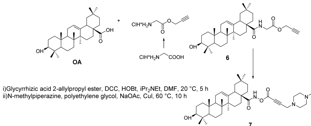
Fig. 4 Synthesis of OA derivatives 6 and 7.
