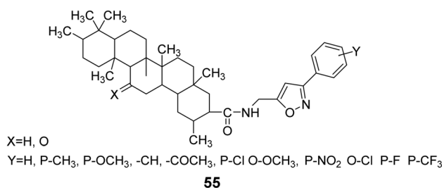
Fig. 17 The structure of isoxazole heterocyclic derivatives 55 of glycyrrhetic acid and dehydroglycyrrhetic acid.
