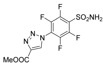
Methyl 1-(2,3,5,6-tetrafluoro-4-sulfamoylphenyl)-1H-1,2,3-triazole-4-carboxylate
