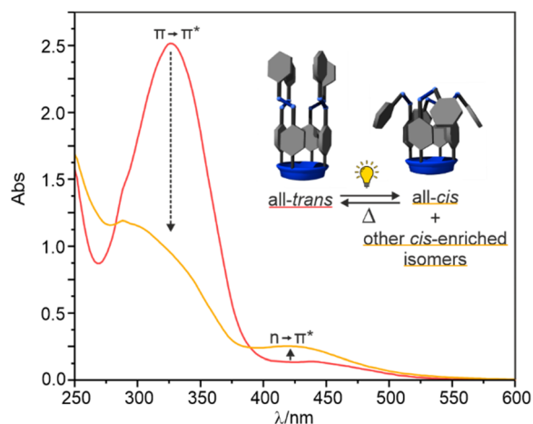
Fig. 2 UV-Vis spectra of a 100 μM DCM solution of 3 before and after light irradiation ( \lambda_{\text{exc}} = 365 nm). The observed changes in the spectra are diagnostic of trans -to- cis isomerization of the azobenzene group. Red line – thermo-equilibrated sample; Orange line – PSS.
