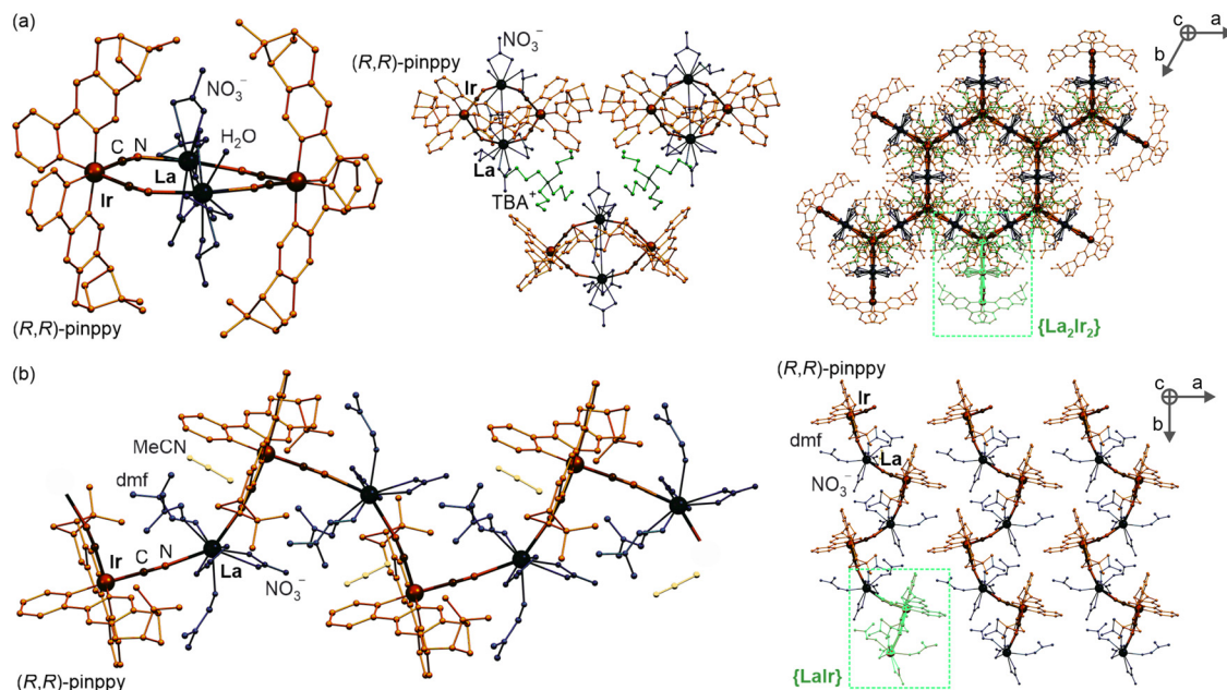
Fig. 2 The representative views on the crystal structures of 3 (a), including the tetranuclear molecule (left part, without TBA + cations that were omitted for clarity), the alignment of these molecules and organic counter-ions (middle part), and the broader view on the supramolecular framework along the six-fold axis, on which one tetranuclear molecule is highlighted in light green (right part), and the view on the crystal structure of 4 (b), including the fragment of a coordination polymer together with solvent molecules of crystallization (left part) and the arrangement of these coordination chains, on which the dinuclear molecular unit is highlighted in light green (right part). The chiral ligand, heavy atoms, cyanido ligands, solvent molecules, and counter-ions are labeled.
