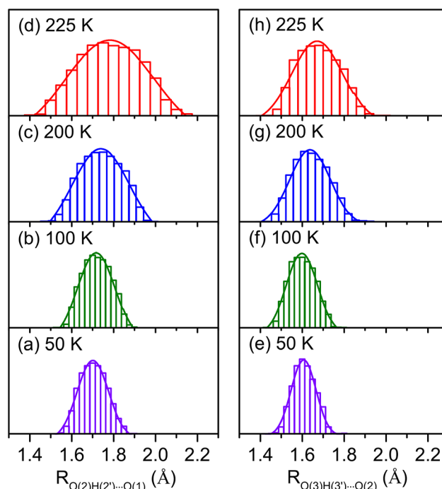
Fig. 4 Normal distribution of O(2)H(2')...O(1) and O(3)H(3')...O(2) hydrogen-bond distances ( R_{O(2)H(2')\cdots O(1)} and R_{O(3)H(3')\cdots O(2)} ) during AIMD simulations of isomer 2-I for HALOH(H 2 O) 2 at 50 K, 100 K, 200 K, and 225 K. The atom labelling is indicated in Fig. 2.
