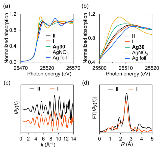
Fig. 3 Solid-state Ag K-edge XAFS measurements of II and I performed at -263 °C. (a) Wide view and (b) enlarged view around the white line ( E = \text{ca. } 25\,512 eV) of XANES spectra. (c) k^3 -Weighted k -space EXAFS spectra and (d) Fourier-transformed R -space EXAFS spectra ( k range, 3–16 Å).
