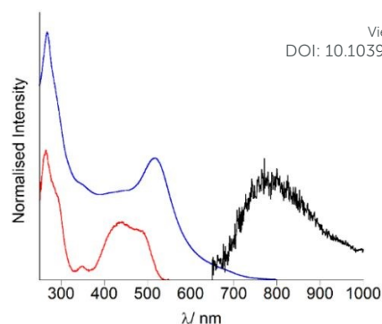
Figure 3. Monitoring OsPhenSS coating on AuNP13 and optical spectra of isolated OsPhen•AuNP13 in water. (a) Titration of 5 \mu L quantities of 1 mM OsPhenSS (5 \mu L aliquots of 1 mM) into 4.5 nM Z•AuNP13 (4.5 nM) in aerated water and (b) isolated OsPhen•AuNP13 UV-Vis absorption spectrum: blue, excitation spectrum ( \lambda_{em} = 770 nm): red, and luminescence emission spectrum ( \lambda_{exc} = 488 nm), black.
