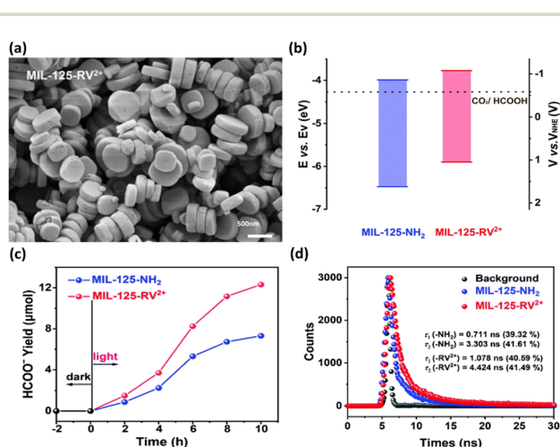
Fig. 4 (a) SEM image of MIL-125-RV 2+ . (b) Band structure of MIL-125-NH 2 and MIL-125-RV 2+ concerning the redox potential of CO 2 /HCOOH at pH = 7. (c) Results of photocatalytic CO 2 reduction under visible light illumination over MIL-125-NH 2 and MIL-125-RV 2+ . (d) Time-resolved PL spectra of MIL-125-NH 2 and MIL-125-RV 2+ . Reproduced with permission from ref. 41. Copyright 2022, Royal Society of Chemistry.
