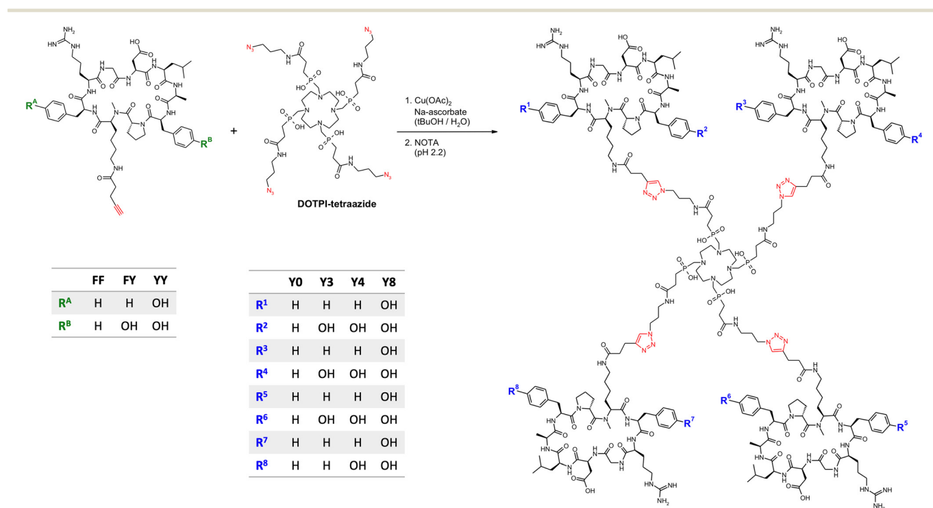
Fig. 2 Synthesis of tetrameric conjugates of \alpha v\beta 6 -integrin binding peptides. Synthesis of Y0 , Y4 , and Y8 was done by reacting DOTPI-tetraazide with the peptides FF , FY , and YY , respectively. The asymmetrical conjugate Y3 was isolated from the CuAAC reaction of DOTPI-tetraazide with a mixture of FF and FY by means of preparative HPLC. Functional groups related to the CuAAC are highlighted in red.
