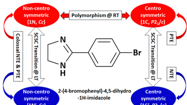
Fig. 16 Polymorphism, phase transition, and unusual thermal expansion characteristics in halogen derivatives of 4-phenyl substituted imidazoline. 168
