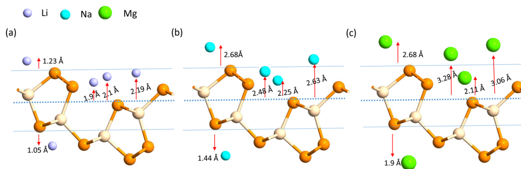
Fig. 3 Adsorption distance of the (a) Li, (b) Na and (c) Mg ions.
