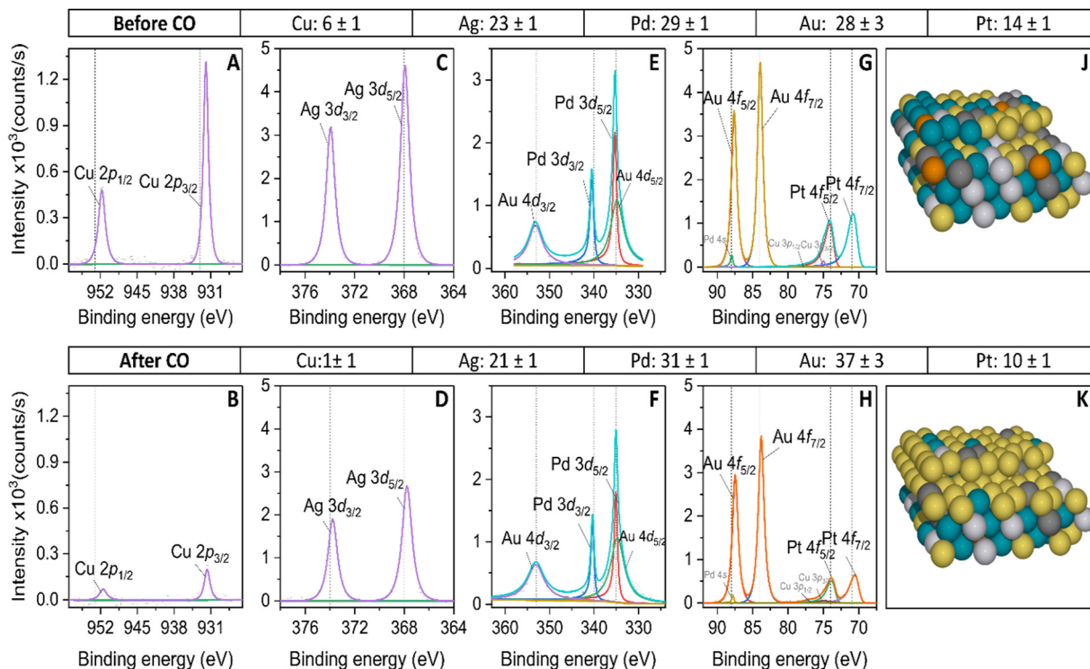
Fig. 5 XPS spectra of scan of the (A) and (B) Cu 2p, (C) and (D) Ag 3d, (E) and (F) Au 4d/Pd 3d, and (G) and (H) Au 4f/Pt 4f peaks of the extended AgAuCuPdPt HEA before and after continuous CO oxidation. All spectra have been background-subtracted (Shirley-type background). (J) and (K) Schematic representation of the HEA surface before and after continuous CO oxidation.
