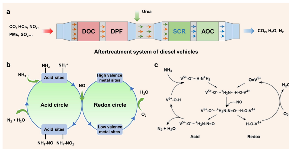
Fig. 1 (a) The after-treatment system of diesel vehicles. (b) Efficient methods for enhancing the acid cycle and redox cycle over de- \text{NO}_x catalysts. (c) The catalytic reaction diagram revealing the double cycles of the \text{NH}_3 -SCR process over vanadia/titania catalysts. Copied with permission from ref. 32. Copyright 1995, Elsevier.
