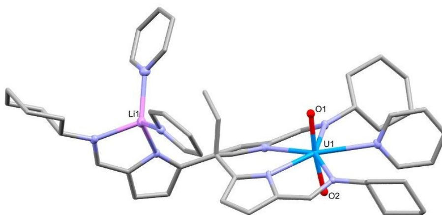
Figure 2. X-ray crystal structure of [\text{UO}_2(\text{py})\{\text{Li}(\text{py})_2\}(\text{L})] ( 3-Li ). For clarity, hydrogen atoms are omitted and displacement ellipsoids of the heteroatoms are drawn at 50% probability. Selected bond distances (Å) and angles (°): U1-O1 = 1.769(3), U1-O2 = 1.772(2), O1-U1-O2 = 173.1(1)°.
