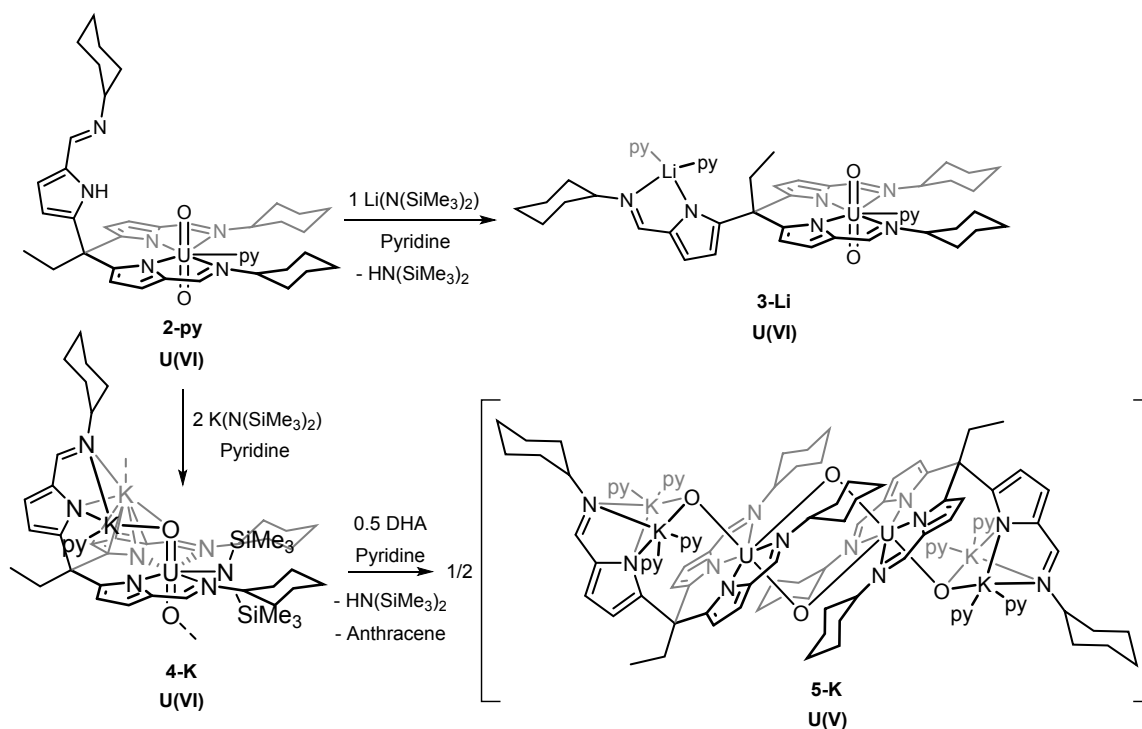
Scheme 2. Synthetic procedures to form [\text{UO}_2(\text{LiL})(\text{py})_3] ( 3-Li ), [\text{UO}_2 and the dimeric, singly-reduced [\text{UO}_2(\text{K}_2\text{L})(\text{py})_4]_2 ( 5-K ).
