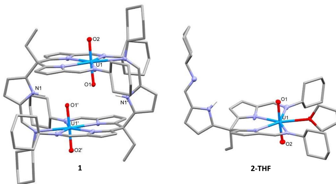
Figure 1. X-ray crystal structures of [\text{UO}_2(\text{HL})]_2 ( 1 , left) and the solvated complex [\text{UO}_2(\text{HL})(\text{THF})] ( 2-THF , right). For clarity, all hydrogen atoms except the pyrrole NH are omitted and displacement ellipsoids of the heteroatoms are drawn at 50% probability. Selected bond distances (Å) and angles (°): 1 , U1-O1 = 1.774(2), U1-
