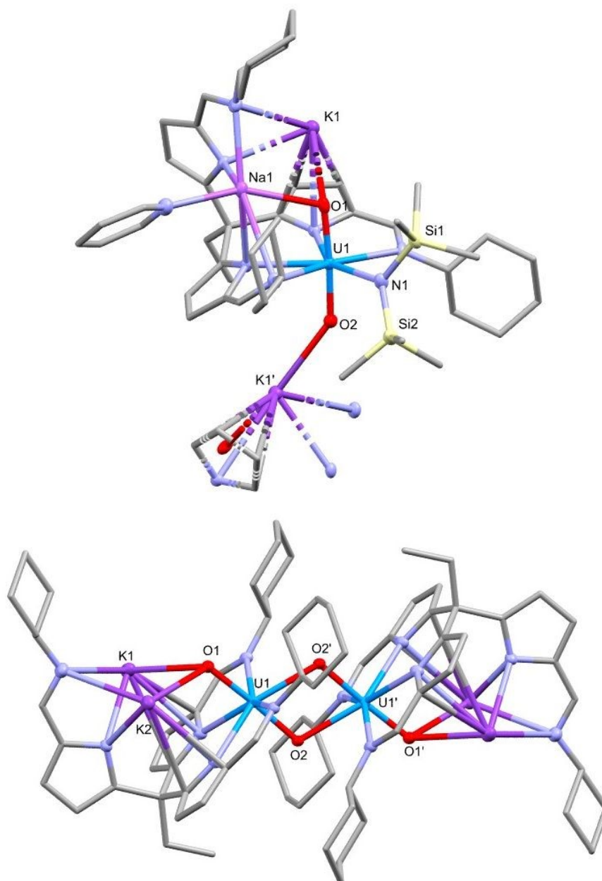
Figure 3. X-ray structures of the U(VI) ( 4-Na/K ), and U(V) ( 5-K ), alkali metal complexes. For clarity, hydrogen atoms are omitted along with the eight pyridine molecules coordinating to the potassium atoms on 5-K ; displacement ellipsoids of the heteroatoms are drawn at 50% probability. Selected bond distances (Å) and angles (°): 4-Na/K , U1-O1 = 1.798(5), U1-O2 = 1.788(5), O1-K1 = 2.900(5), O2-K1' = 2.772(5), O1-U1-O2 = 175.8(2); 5-K , O1-U1 = 1.872(2), O2-U1 = 1.936(2), U1-O2' = 2.377(2), K1-O1 = 2.927(2), K2-O1 = 2.806(2), U1-U1' = 3.4993(5), O1-U1-O2 = 177.33(9), O1-U1-O2' = 110.70(9), O2-U1-O2' = 71.96(8).
