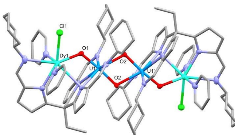
Figure 5. X-ray crystal structure of complex 6-Dy . For clarity, hydrogen atoms are omitted and displacement ellipsoids of the heteroatoms are drawn at 50% probability. Selected bond distances and angles are shown in Table 1.
