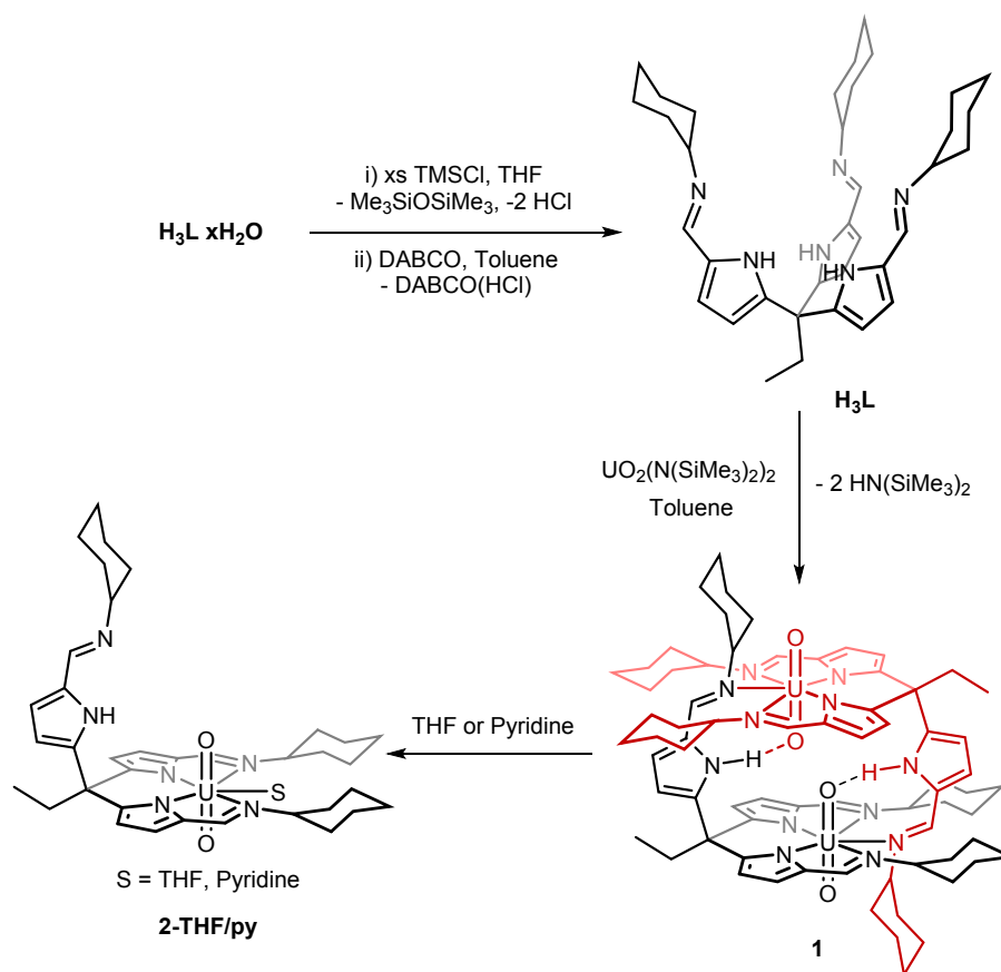
Scheme 1. Synthetic procedures to form [\text{UO}_2(\text{HL})]_2 ( 1 ) and the solvated [\text{UO}_2(\text{HL})(\text{THF})] ( 2-THF ) and [\text{UO}_2(\text{HL})(\text{py})] ( 2-py ) uranyl(VI) complexes. For clarity the separate ligand moieties of 1 have been displayed in black and red.
