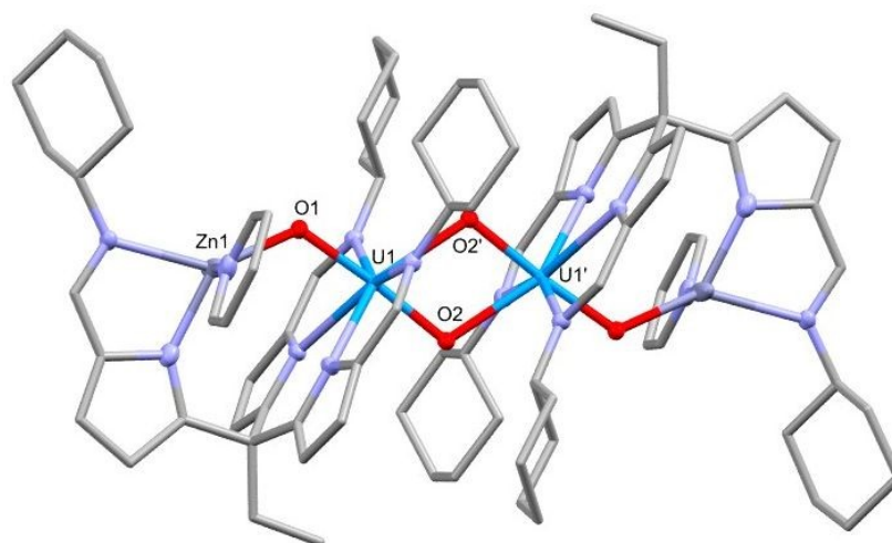
Figure 4. X-ray structure of 6-Zn. For clarity, hydrogen atoms are omitted and displacement ellipsoids of the heteroatoms are drawn at 50% probability. Selected bond distances (Å) and angles (°): U1-O1 = 1.929(2), U1-O2 = 1.939(2), U1-O2' = 2.349(1), Zn1-O1 = 1.964(1), Zn1-U1 = 3.4037(5), U1-U1' = 3.4862(5), O1-U1-O2 = 176.18(6), Zn1-O1-U1 = 121.97(7). Each zinc centre has essentially 1.5 pyridine ligands, one was modelled as half-occupied, consistent with disorder imposed by space group symmetry, and is not shown for clarity.
