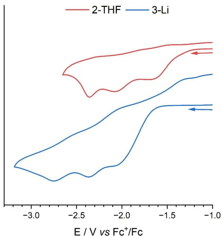
Figure 8. Cyclic voltammogram of complexes 2-THF (RED) and 3-Li (BLUE). A glassy-carbon working electrode, platinum counter electrode and silver wire pseudo-reference electrode were used with a 10mM solution of analyte in 0.1 M THF solutions of [\text{nBu}_4\text{N}][\text{PF}_6] electrolyte. Voltammograms were recorded under a dinitrogen atmosphere in a glovebox at a scan-rate of 0.1 \text{ V s}^{-1} .
