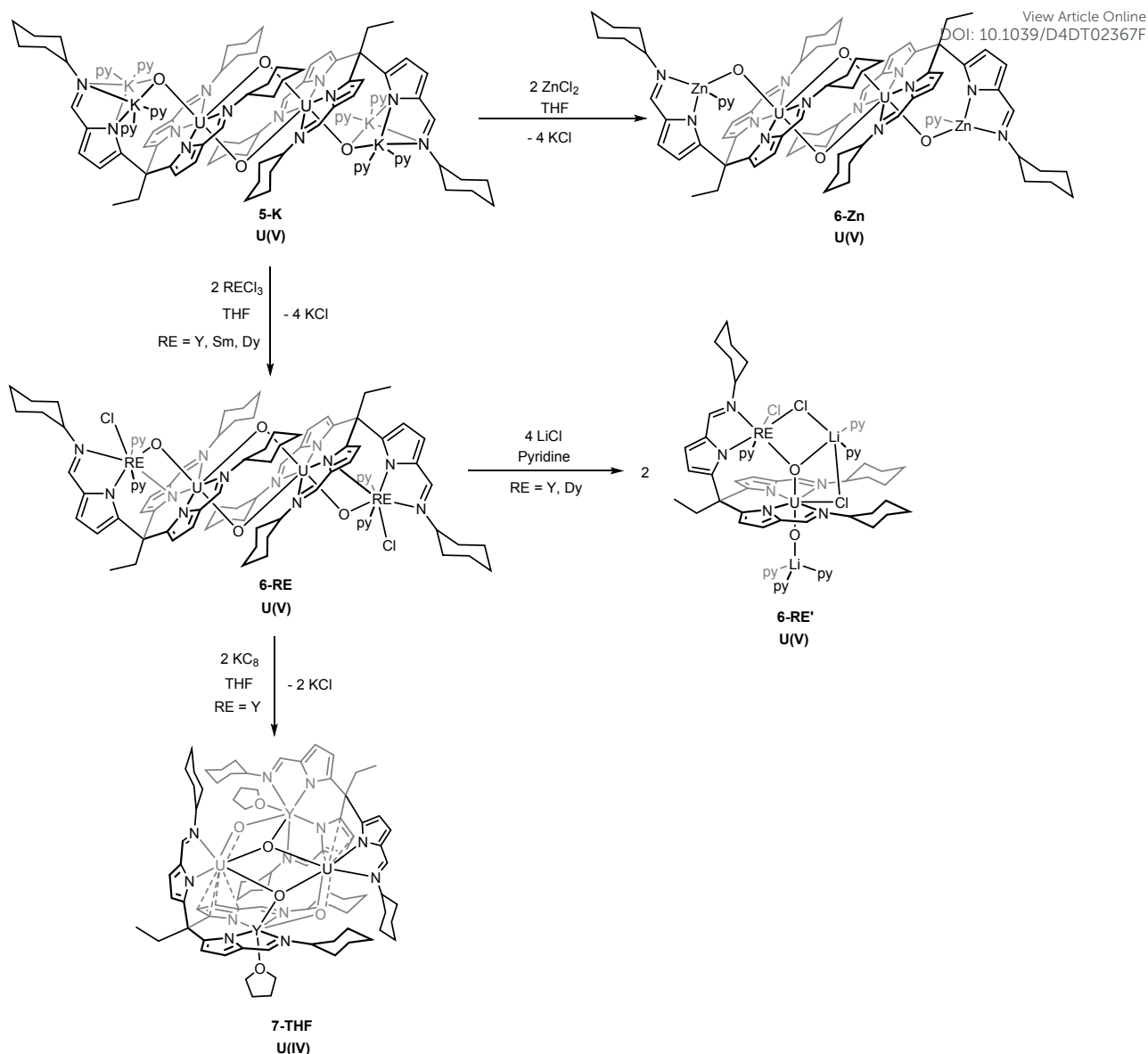
Scheme 3. Synthetic procedures to the formation of the U(V) heterobimetallic complexes [\text{UO}_2(\text{ZnL})_2] (6-Zn), and [\text{UO}_2(\text{REL})(\text{Cl})_2] (6-RE) by reaction of 5-K with the respective metal chloride; [\text{UO}_2(\text{RE})(\text{Cl})(\text{LiCl})_2] (6-RE') by the treatment of 6-RE with four equivalents of LiCl; and the dimeric U(IV) complex [\text{UO}_2(\text{YL})(\text{THF})_2] (7-THF), by the reduction of 6-Y with two equivalents of \text{KC}_8 .
