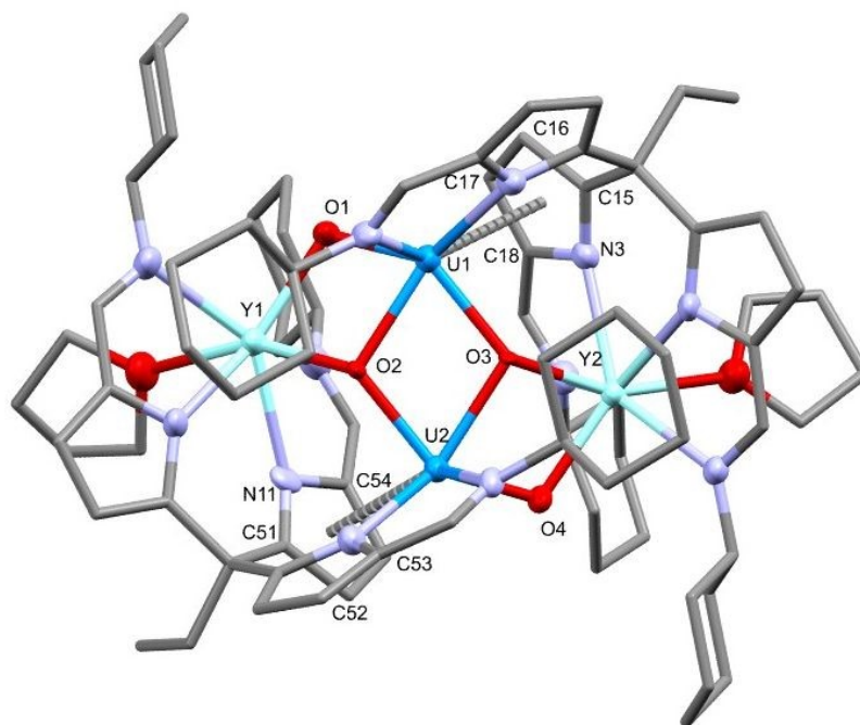
Figure 7. X-ray structure of the U(IV) yttrium-uranium hetero-tetrametallic complex 7-THF. For clarity, hydrogen atoms are omitted and displacement ellipsoids of the heteroatoms are drawn at 50% probability. Selected bond distances (Å) and angles (°): U1-O1 = 2.042(7), U1-O2 = 2.250(5), U1-O3 = 2.175(6), U2-O2 = 2.175(6), U2-O3 = 2.245(5), U2-O4 = 2.044(5), Y1-O1 = 2.218(6), Y1-O2 = 2.204(6), Y2-O3 = 2.203(5), Y2-O4 = 2.212(6), Y1-U1 = 3.469(1), Y2-U2 = 3.4583(8), U1-U2 = 3.5856(5), U1-N3 = 3.091(8), U1-C15 = 3.09(1), U1-C16 = 3.00(1), U1-C17 = 3.011(9), U1-C18 = 3.06(1), U2-N11 = 3.058(8), U2-C51 = 3.05(1), U2-C52 = 2.955(8), U2-C53 = 2.971(8), U2-C54 = 3.009(9), O1-U1-O3 = 136.3(2), O2-U2-O4 = 137.7(2).
