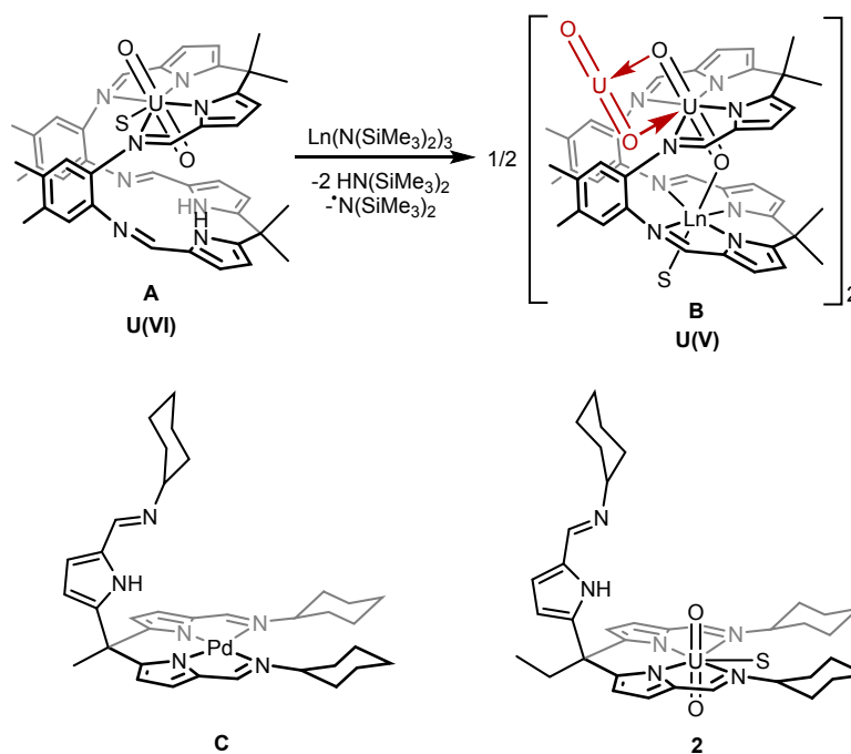
Chart 1. Top: Example of the reaction of a uranyl “Pacman” complex ( A ) and a lanthanide silylamide to form the Ln-functionalised uranyl(V) complex ( B ) via ligand deprotonation and radical transfer. 19, 20 Bottom: The “Hangman” palladium complex C (previous work) and uranyl complex 2 (this work) in which two ligand “arms”
