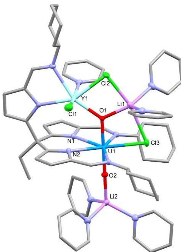
Figure 6. X-ray crystal structure of the monomeric rare-earth-uranium(V) complex 6-Y' . For clarity, hydrogen atoms are omitted and displacement ellipsoids of the heteroatoms are drawn at 50% probability. Selected bond distances and angles are shown in Table 2.
