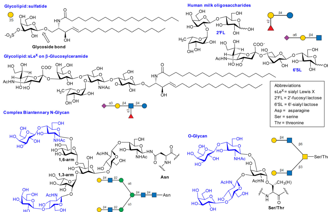
Fig. 2 Selected examples of lectin ligands. SNFG nomenclature was generated using glycoGlyph. 8 The N-glycan and O-glycans shown are bivalent glycoclusters where two LacNAc disaccharides (blue) are presented on saccharide scaffolds (black).
