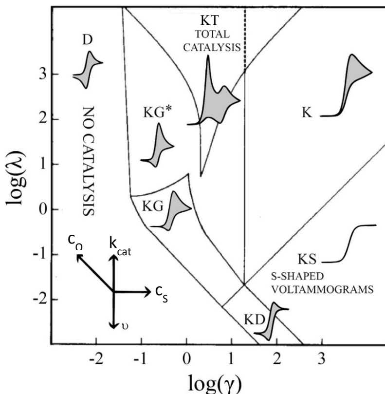
Figure 6: Diagram of the catalytic zones for simulated CVs of one electron reduction of substrate S via a redox mediator, O . The kinetic parameter \lambda = \left(\frac{RT}{F}\right)\left(\frac{k_{\text{Cat}}c_O}{\nu}\right) and the excess factor \gamma = \frac{c_S}{c_O} represent the competition between catalytic rate and scan rate, and the initial electrolyte composition, respectively. The CV waveforms follow the convention of negative potentials to the right and cathodic current upward. Scans are started from positive potentials. Reprinted with permission from ref 38 Copyright 2014 American Chemical Society.
