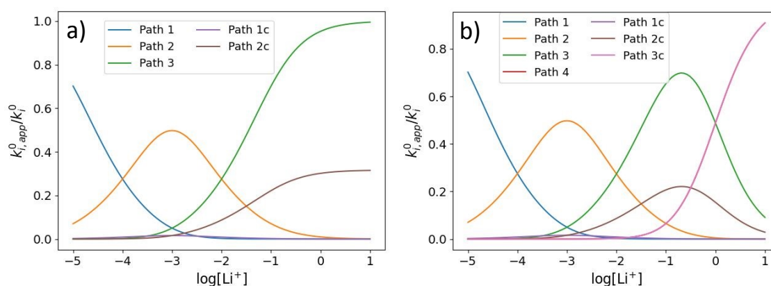
Figure 3: Example of behaviour of the apparent standard rate constant for each of the pathways represented in Scheme 1a with n=2 (a) and n=3 (b). The plots shown in the figures were computed using the parameters K_{a1}^R=1 \times 10^5 , K_{a2}^R=1 \times 10^3 , K_{a1}^O=1000 , K_{a2}^O=10 , and K_{a3}^R=K_{a3}^O=0 for (a) and K_{a3}^R=K_{a3}^O=1 for (b). The parameters were chosen so that the behaviour of the different pathways can be seen clearly. The actual positions and magnitudes of the curves' maxima and plateaus strongly depend on these parameters, but their shapes are characteristic of the different paths.
