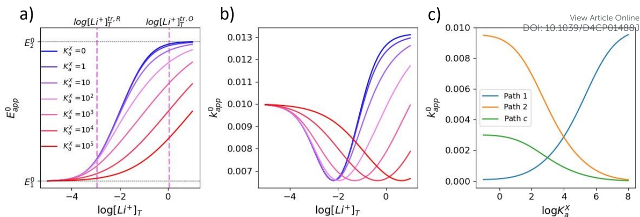
Figure 5: Variation of apparent standard potential (a) and total rate constant (b) with supporting salt concentration for different values of supporting salt association constant, K_a^X varying between 0 and 10^5 . Vertical pink dashed lines represent the transition concentrations for the case of K_a^X = 100 , corresponding to the pink curve, as an example. (c) Variation of the contribution of each pathway with change in K_a^X . The plots in the figures were computed using K_a^O=10 , K_a^R=1000 , k_1^O=k_2^O=k_c^O=0.01 for (a) and (b), and [Li^+]_T = 1M for (c).
