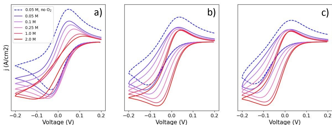
Figure 7: Simulated cyclic voltammograms for each of the DBBQ reduction pathways depicted in Scheme 2, pathways a) 1, b) 2, and c) c, followed by reaction of DBBQ with oxygen according to equations (3) and (6). The three plots are computed using K_a^O=2 , K_a^R=10 , k_1^O=k_2^O=k_3^O=0.01 cm/s, k_4=50 and k_5=10^{10} , and a scan rate of 50 mV/s at different \text{Li}^+ concentrations as stated in the legend. A simulated CV in the absence of \text{O}_2 and 0.05 M \text{Li}^+ is also shown for comparison, depicted by the blue dashed lines.
