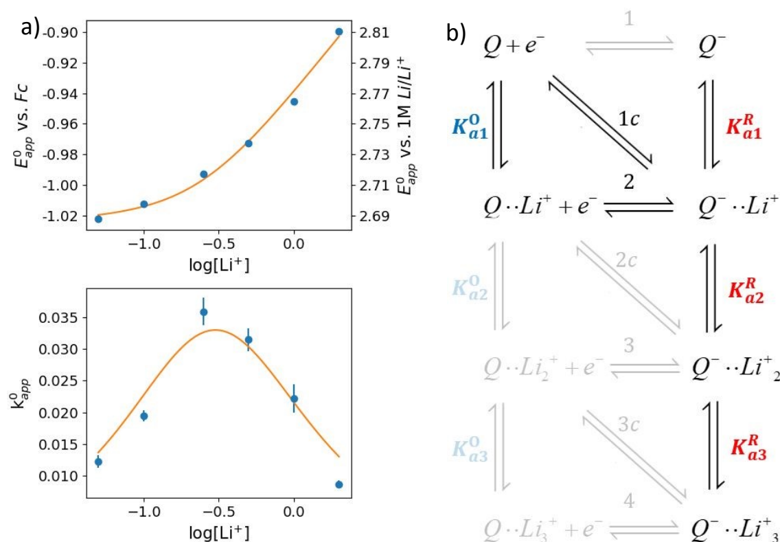
Figure 4: a) experimental standard potential, E^0 (top) and kinetic constant, k^0 (bottom) represented as dots compared with the fitting results when assuming the mechanism represented in panel b). The values derived from the fits are given in Table 1. b) Schematic of the possible pathways for redox activity of DBBQ in \text{Li}^+ containing DMSO solutions. The greyed-out pathways were not needed to explain the experimental behaviour.
