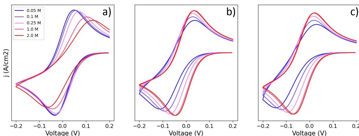
Figure 2: Simulated cyclic voltammograms for each of the pathways depicted in Scheme 2: pathways, a) 1, b) 2, and c) c. The three plots are computed using K_a^0=2 , K_a^R=10 and k_1^0=k_2^0=k_3^0=0.01 , all with a scan rate of 50 mV/s and [Q]=5\text{mM} , for [Li^+] ranging from 0.05 – 2M.
