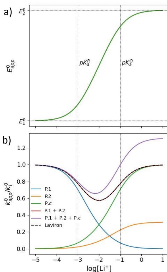
Figure 1: a) Evolution of apparent potential of the system as a function of lithium concentration. b) Evolution of individual components of the normalized rate constant and total rate constant as a function of lithium concentration. P.1, P.2, and P.c represent Pathways 1, 2 and c, respectively. The black dashed line corresponds to the expression obtained by Laviron 27 for the total kinetic constant, considering pathways 1 and 2, k_{1,app}^0 + k_{2,app}^0 (see text in section 1.2 for definition), assuming \alpha_1 = \alpha_2 = 0.5 . Figures were computed using K_a^O=10 , K_a^R=1000 , k_1^0 = k_2^0 = k_3^0 = 0.01 .
