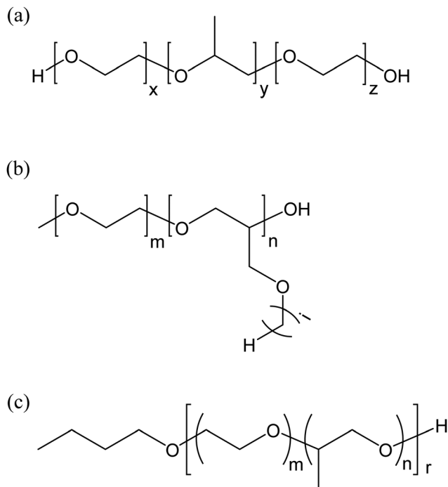
Fig. 10 Structures of three nonionic amphiphilic polymers. (a) Polyoxoethylene-co-polyoxopropylene-co-polyoxoethylene; (b) polyoxoethylene-co-poly(alkylglycidyl ether); (c) random polyoxoethylene-co-polyoxopropylene monobutyl ether.
