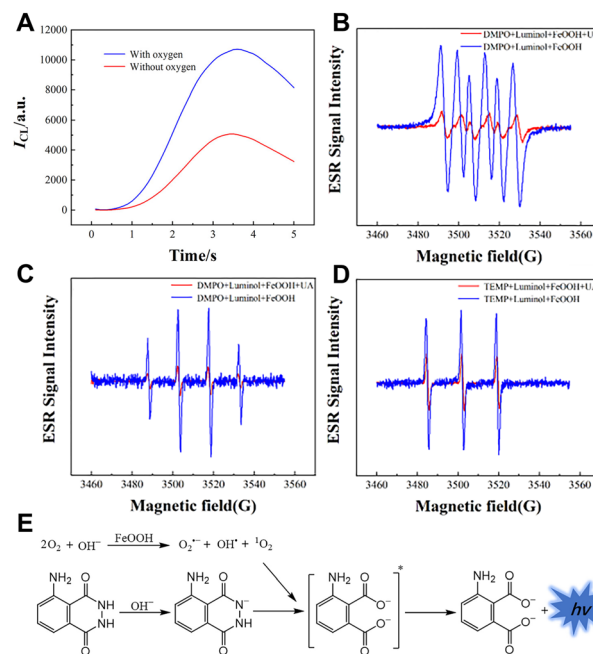
Fig. 12 (A) CL kinetic curves of the luminol/FeOOH system in the absence and presence of oxygen. ESR spectra of adducts. (B) DMPO-O 2 • - (C) DMPO-OH• and (D) TEMP-O 2 • - in the luminol/FeOOH CL system. (E) Mechanism of the luminol/FeOOH CL system. [Luminol]: 100 μM; [FeOOH]: 25 μg mL -1 ; [UA]: 5 μM; [pH]: 10.0. Reprinted with permission from ref. 63, Copyright 2023 American Chemical Society.
