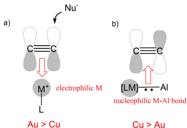
Scheme 9 (a) Electrophilic behaviour of [\text{LM}]^+ ( M = \text{Cu}, \text{Au} ) complexes for alkyne activation (Au more efficient than Cu); (b) nucleophilic behaviour of the M–Al ( M = \text{Cu}, \text{Au} ) bond in coinage metal–aluminyl complexes towards alkynes (Cu more efficient than Au).
