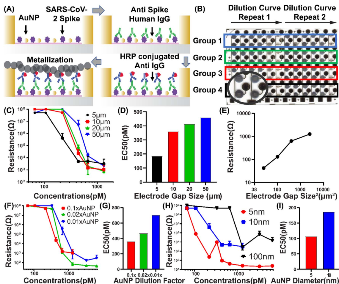
Fig. 3 (A) Schematic of assay workflow. (B) Optical image of the chip after metallization. \mu IDEs with four different gaps are fabricated on the same chip, indicated here as: black: 5 \mu\text{m} , red: 10 \mu\text{m} , green: 20 \mu\text{m} , blue: 50 \mu\text{m} . Inset shows zoomed-in view of \mu IDEs. (C and D) Resistance reading and EC50 from dilution curves of anti-S mAb using 1:10 \times 10 nm AuNP across different electrode gaps. (E) Resistance versus square of electrode gap at 1.33 nM of anti-S mAb. (F and G) Resistance reading and EC50 from dilution curves of anti-S mAb using 10 nm AuNP on 5 \mu\text{m} electrode gaps across different AuNP concentrations. (H and I) Resistance reading and EC50 from dilution curves of SARS-CoV-2 spike antibody using 0.1 \times AuNP on 5 \mu\text{m} electrode gaps with different AuNP diameters. Each group has a repeat number n = 2 , standard deviations are shown as error bars.
