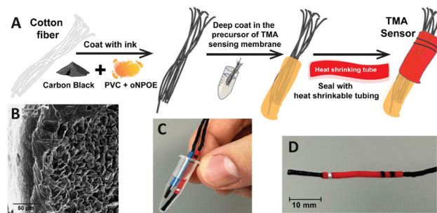
Fig. 4 (A) The process of preparing a home-made TMA sensor for vaginosis analysis. (B) A SEM cross-section image of the membrane coated TMA sensor (scale bar is 50 \mu\text{m} ). (C and D) Photographs of the sensor depicting its portability and size. 102 Copyright 2023, MDPI.
