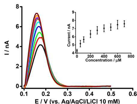
Fig. 5 DPVs at different concentrations of \beta -CD at fixed concentrations of BSA ( 0.6 \text{ mM} ) and PFOA ( 50 \mu\text{M} ) at the \mu\text{TIES} array. Cell composition as given in Scheme 1. Black, red, green, blue, cyan, dark yellow, violet, orange, and wine red, respectively, represent the DPVs at 50, 100, 200, 300, 400, 500, 600, and 700 \mu\text{M} \beta -CD. Inset: relationship between peak current and concentration of \beta -CD. DPVs were background-subtracted followed by baseline-corrected. Error bars indicate \pm 1 standard deviation from two independent measurements.
